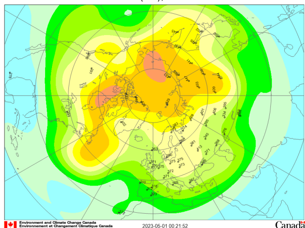
Mean total ozone (DU), 2023/04/01-2023/04/30
