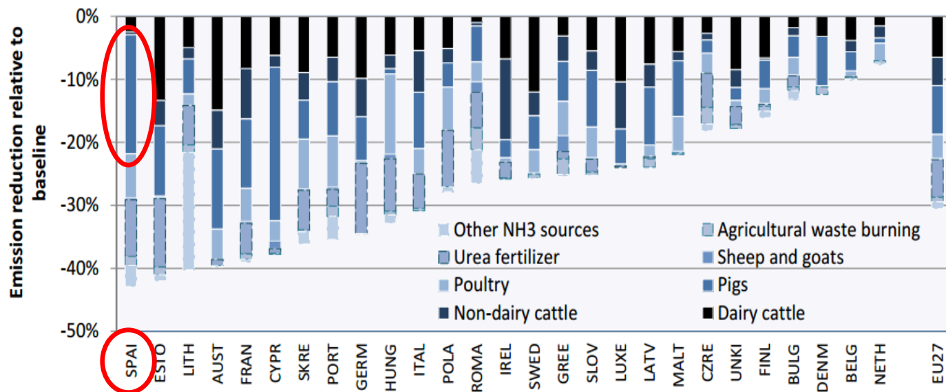
Figure 5.15: Mitigation potentials for NH 3 emissions in 2030 on top of current legislation
